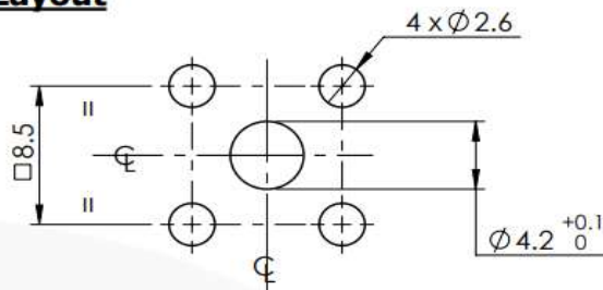
Hole Layout
