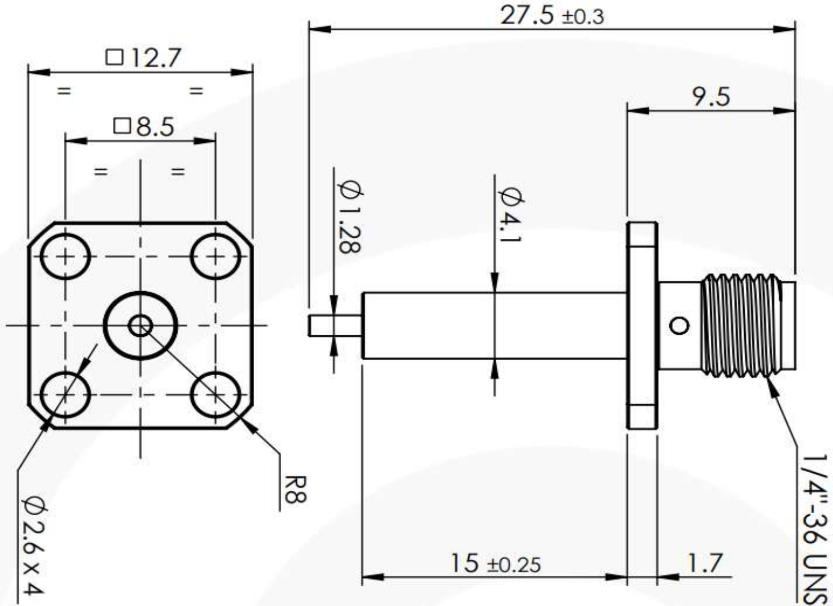
Hole Layout
