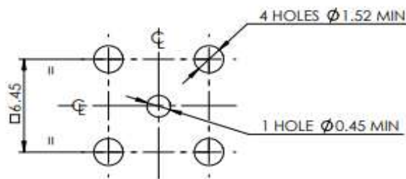
Recommended Hole Layout
