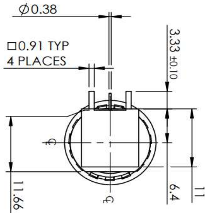
Recommended Hole Layout
