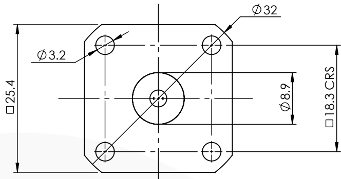
FLANGE MOUNTING HOLES
