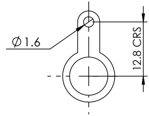
SOLDER TAG DETAILS
