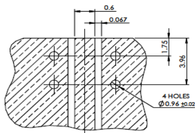
PCB LAYOUT - NOT TO SCALE
