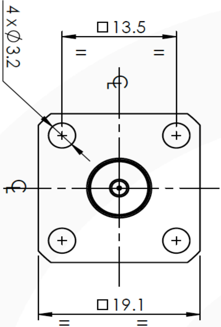
Hole Layout
