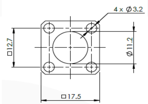
FLANGE MOUNTING HOLES
